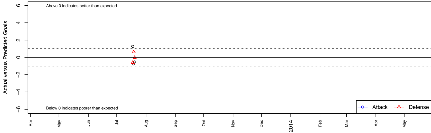
FC Boulder Elite B99 Dots are actual minus expected GF (blue circles) and GA (red triangles). Blue line is smoothed change in attack strength. Red is smoothed change in defense strength.
